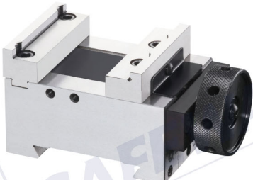
虎鉗滑座 YES VISE ORDER NO.42100002 MODEL: MV-72100CS
