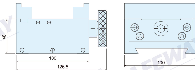
虎鉗滑座 YES VISE ORDER NO.42100006 MODEL: MV-100100PS
