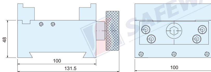
虎鉗滑座 YES VISE ORDER NO.42100004 MODEL: MV-100100CS
